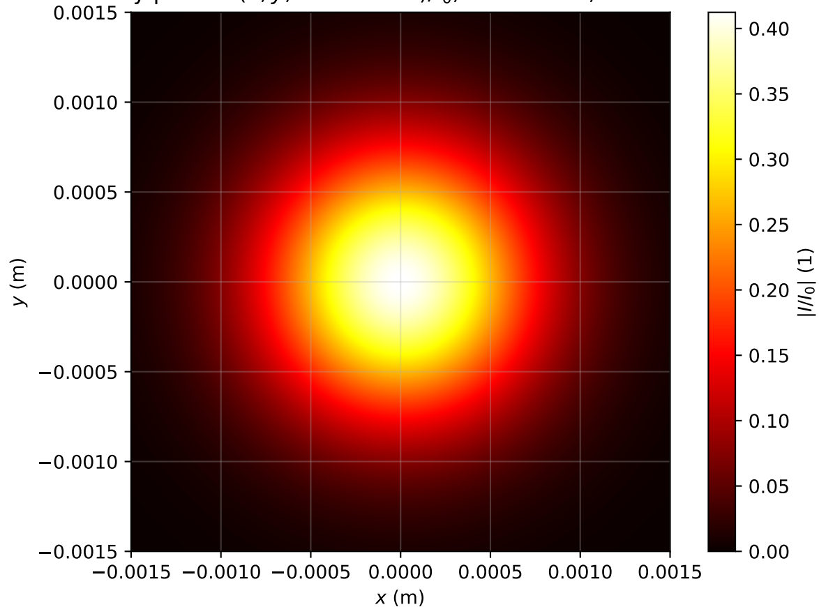
Intensity profile I(x, y, z = 2.786m)/I_0 , P_{in}=0.2P_{cr} , artificial time
